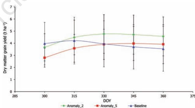
Figure 3. Effects of sowing date on simulated dry matter grain yield of durum wheat under climate change scenarios.
