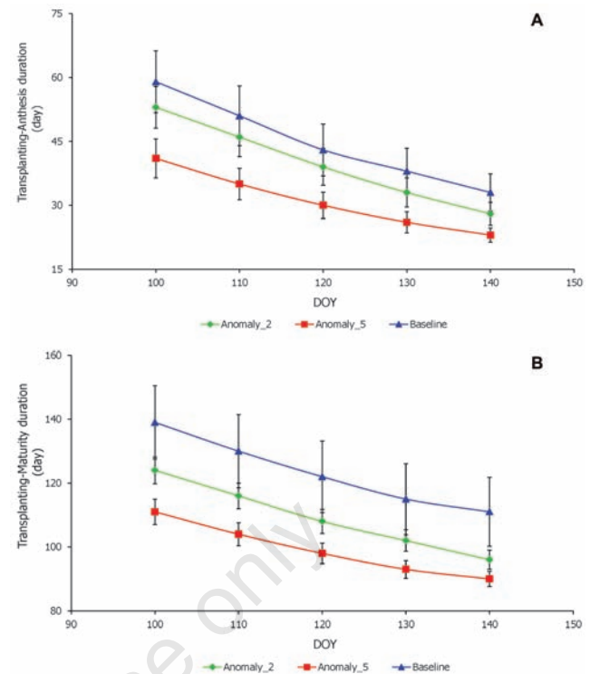
Figure 7. Effects of transplanting date on simulated vegetative (A) and reproductive (B) duration of tomato under climate change scenarios.
