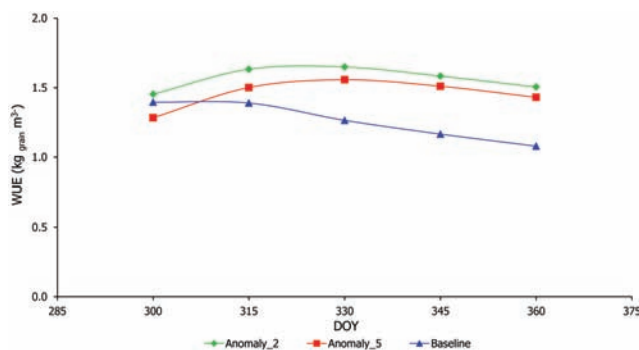
Figure 6. Effects of sowing date on simulated water use efficiency in grain yield of durum wheat under climate change scenarios.
