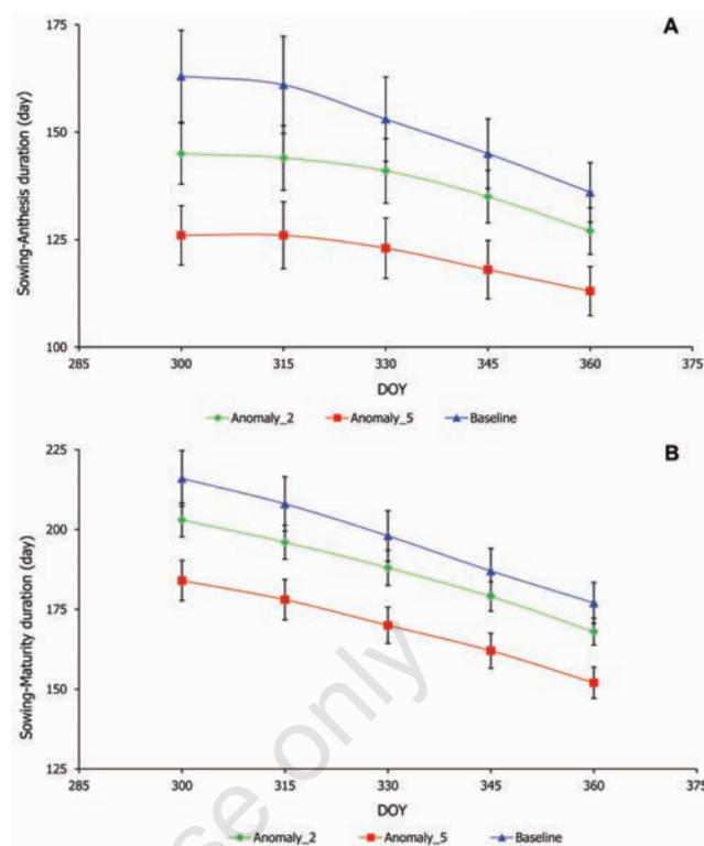
Figure 2. Effects of sowing date on simulated vegetative (A) and reproductive (B) duration of durum wheat under climate change scenarios.
