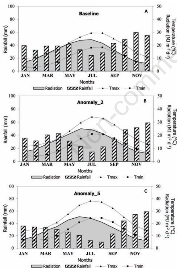
Figure 1. Monthly average of air temperature (maximum and minimum), solar radiation and rainfall of the three scenarios: Baseline (A), Anomaly_2 (B) and Anomaly_5 (C).
