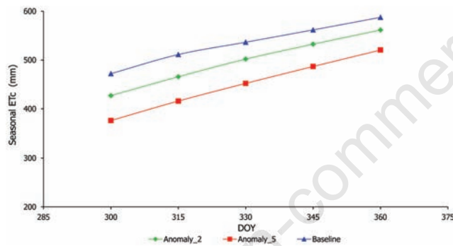
Figure 5. Effects of sowing date on simulated seasonal potential evapotranspiration of durum wheat under climate change scenarios.
