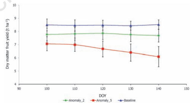
Figure 8. Effects of sowing date on simulated dry matter fruit yield of tomato under climate change scenarios.
