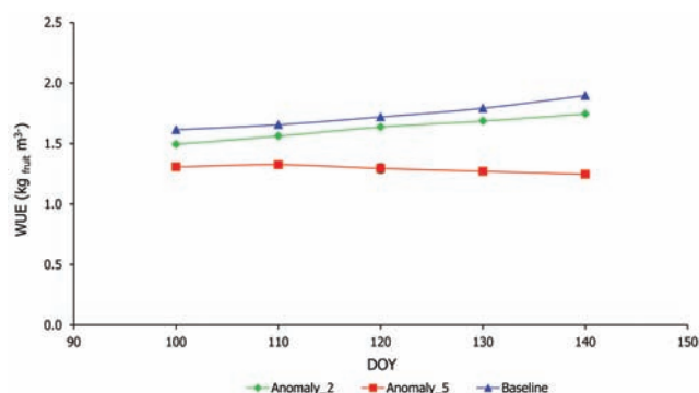
Figure 10. Effects of sowing date on simulated water use efficiency in fruit yield of tomato under climate change scenarios.
