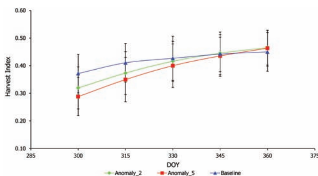
Figure 4. Effects of sowing date on simulated harvest index of durum wheat under climate change scenarios.
