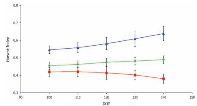
Figure 9. Effects of sowing date on simulated harvest index of tomato under climate change scenarios.
