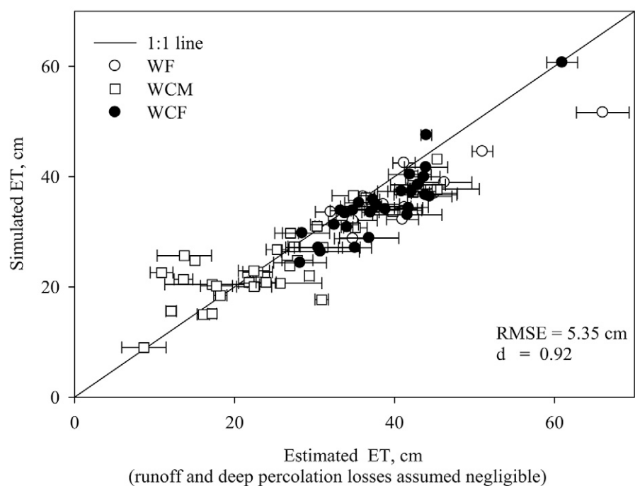
Fig. 9. Measured and simulated crop (winter wheat, corn, and proso millet) evapotranspiration (ET) under wheat–fallow (WF), wheat–corn–fallow (WCF), and wheat–corn–millet (WCM). The error bars indicate one SD of measured means. RMSE = root mean squared error, SD = standard deviation, and d = index of agreement.
