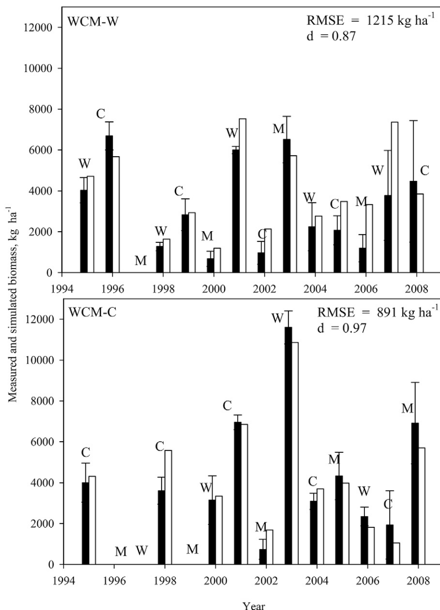
Fig. 3. Comparison of measured (solid bars with error bars) and simulated (open bars without error bars) biomass for wheat, corn and millet grown in the wheat–corn–millet rotation beginning with the wheat phase in 1995 (WCM-W) and beginning with the corn phase in 1995 (WCM-C). The error bars indicate one standard deviation of measured means. RMSE = root mean squared error and d = index of agreement.
