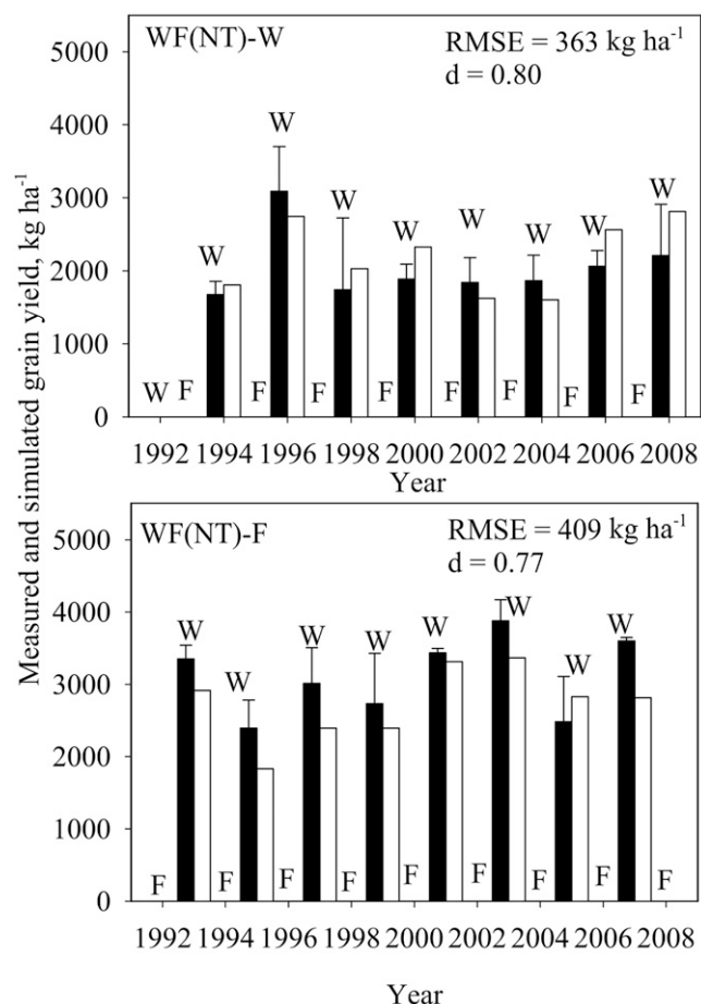
Fig. 5. Measured (solid bars with error bars) and simulated (open bars without error bars) winter wheat yield in the wheat–fallow with wheat phase in 1992 (WF–W) and wheat–fallow with fallow phase in 1992 (WF–F). The error bars indicate one SD of measured means. RMSE = root mean squared error, SD = standard deviation, and d = index of agreement.
