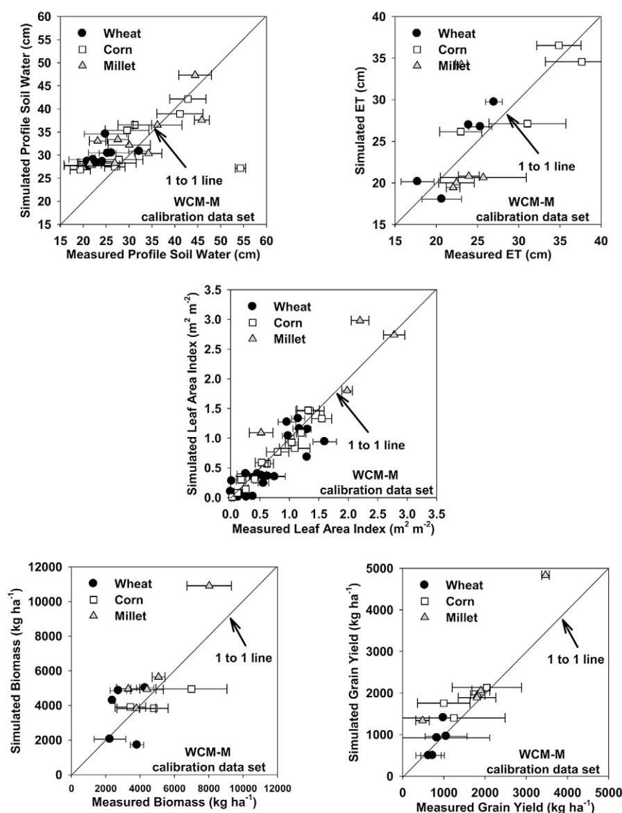
Fig. 1. Comparison of RZWQM2-simulated vs. measured total profile soil water, evapotranspiration, leaf area index, biomass, and grain yield for wheat, corn, and proso millet grown in a wheat–corn–millet rotation at Akron, CO (1995–2008). WCM-M indicates the calibration data set of the wheat–corn–millet rotation beginning with the millet phase in 1995. Error bars indicate one standard deviation from the measured means.
