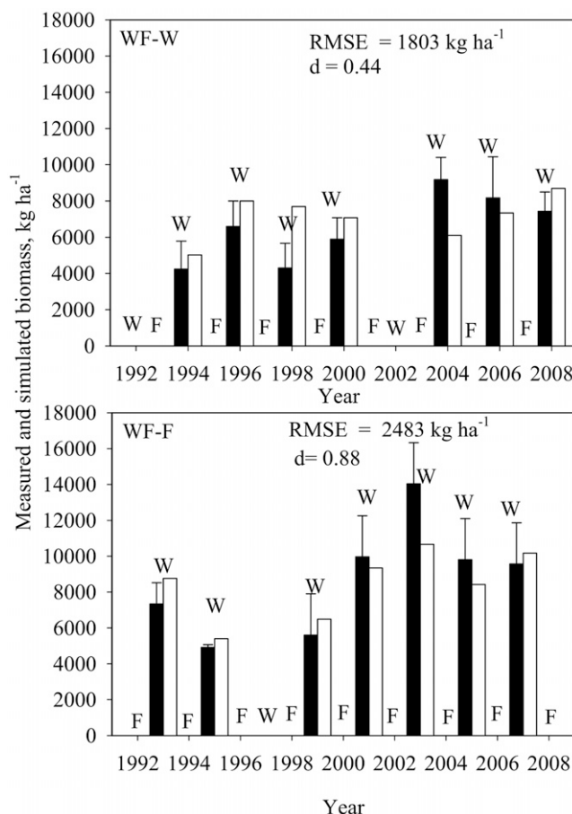
Fig. 6. Measured (solid bars with error bars) and simulated (open bars without error bars) winter wheat biomass in the wheat–fallow with wheat phase in 1992 (WF–W) and wheat–fallow with fallow phase in 1992 (WF–F). The error bars indicate one SD of measured means. RMSE = root mean squared error, SD = standard deviation, and d = index of agreement.
