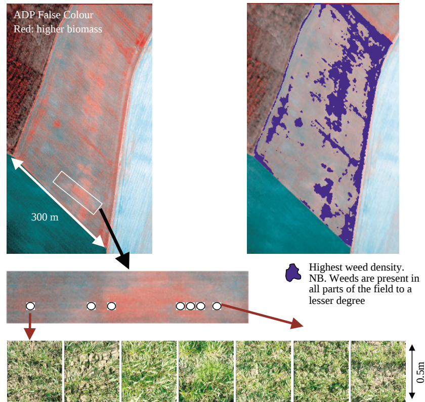
Fig. 19. Weed patches as shown by aerial digital photography (ADP) (after Wood, 2002)
