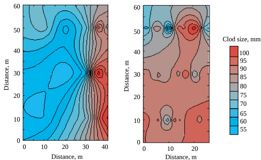
Fig. 11. Clod size maps for two experimental areas, clay (left) and sandy loam (right) (after Bogrekci, 2001)
