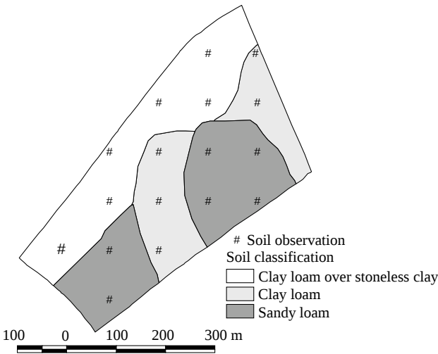
Fig. 2. Soil map based on textural observations sampled at 100m grid (after James et al. , 2000)
