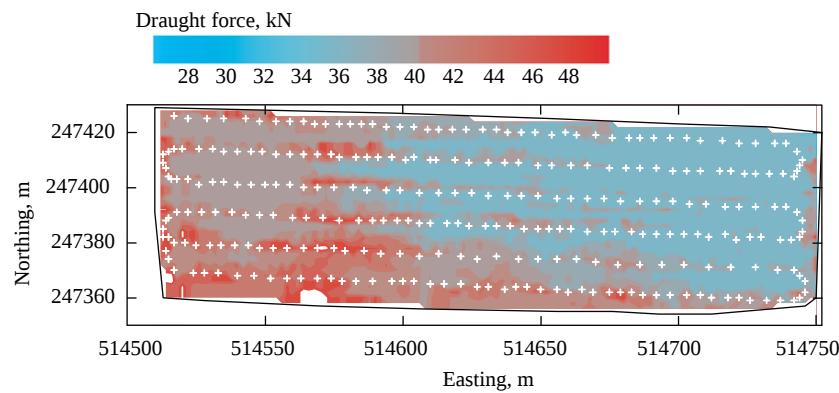
Fig. 9. Subsoiler draught force map showing higher forces commensurate with the compaction caused by tractors operating in the tramlines (shown in white) (after Richards, 2000)
