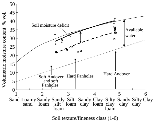
Fig. 4. Volumetric moisture content—soil textural class relationships for electromagnetic induction (EMI) surveys at field capacity and after harvest in Trent Field, (after Waite et al. , 2000): \diamond , February 1999; \square , July 1998; — UK field capacity ( -0.05 bar); ----, UK permanent wilting point ( -15 bar); — —, logarithmic best fit (July 1998); — —, logarithmic best fit (February 1999); soil series, Panholes and Andover
