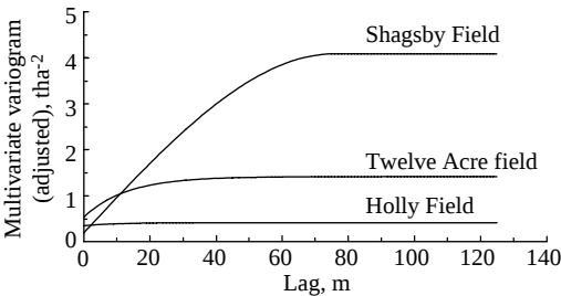
Fig. 1. Semi-variogram of three arable fields (after Lark et al. , 1998)
