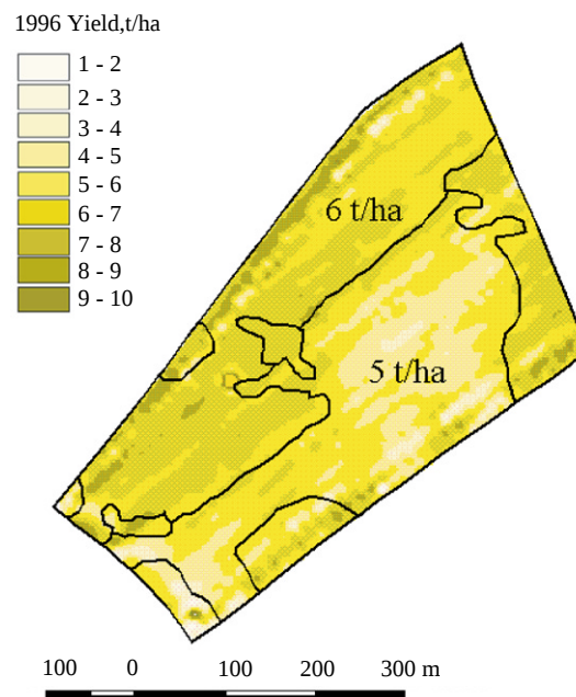
Fig. 7. Average grain yields zone to major soil boundaries from the electro-magnetic induction (EMI) survey (after James et al. , 2000)
