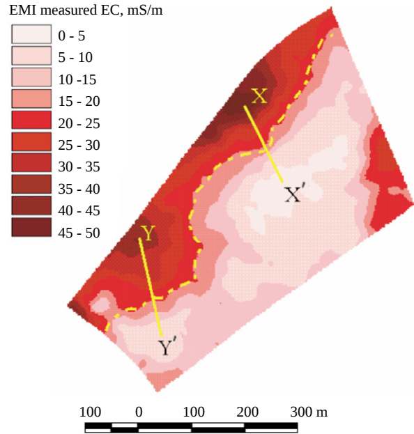
Fig. 5. Map of electrical conductivity (EC) using an electromagnetic induction (EMI) scanner (after James et al. , 2000); XX' and YY', transects
