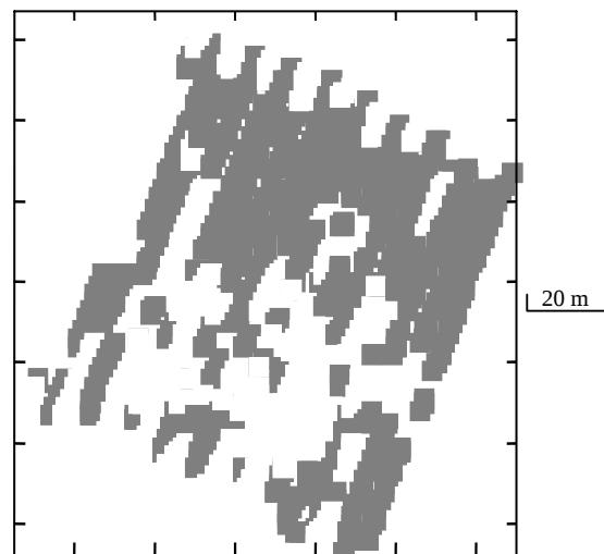
Fig. 18. Wild oat patches mapped with voice recognition system on all terrain vehicle (ATV), January 2000
