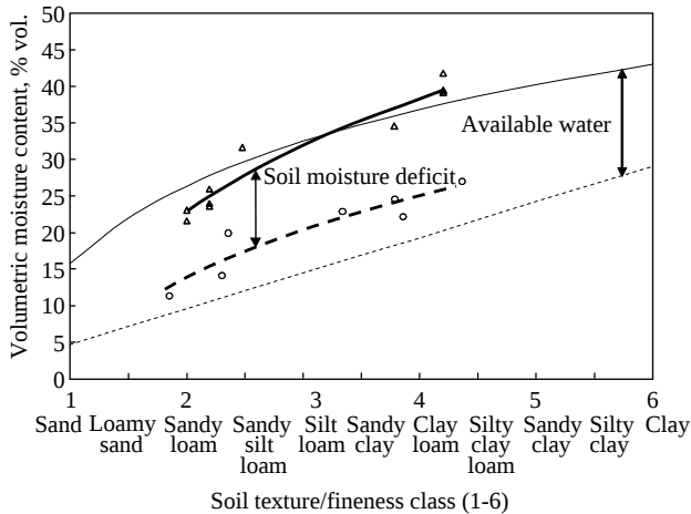
Fig. 3. Volumetric moisture content—soil textural class relationships for electromagnetic induction (EMI) surveys at field capacity and after harvest in the field in Fig. 2 (after Waite et al. , 2000): \Delta , March 1999; \circ , August 1997; — UK field capacity ( -0.05 bar); ---- UK permanent wilting point ( -15 bar); — —, logarithmic best fit (March 1999); — —, logarithmic best fit (August 1997)
