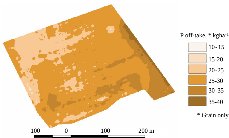
Fig. 15. Application rate for P to replace that removed at harvest
