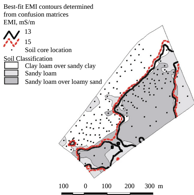
Fig. 6. The detailed soil map, observations on a 24 m grid in the centre section and 50 m grid in the remainder of the field, with the best fit electromagnetic induction (EMI) contours, shown (after James et al. , 2000)
