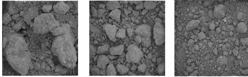
Fig. 12. Images clod size for ploughed soil (left), ploughed and spring tine cultivation (middle) and ploughed and power harrowed (right) (after Bogrecki, 2001)
