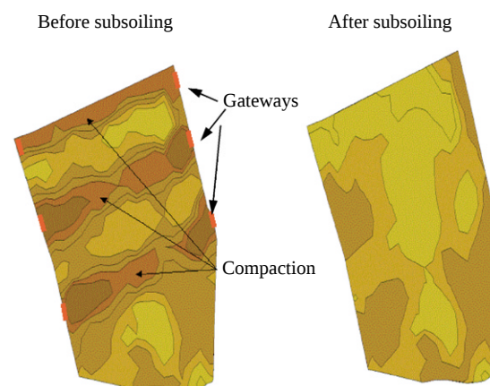
Fig. 8. Electromagnetic induction (EMI) survey showing compaction as a result of farm traffic between gateways to the right and left of the field (left) and the removal of the compaction following subsoiling (right) (after Smith, 2001)
