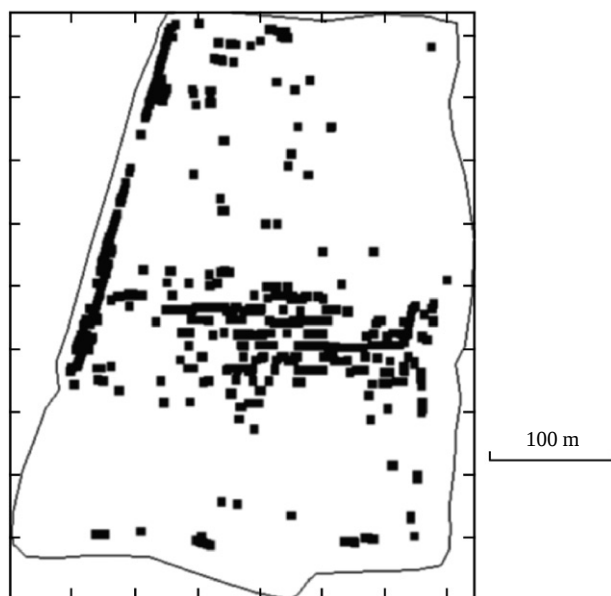
Fig. 17. Wild oat patches mapped from the combine using Fieldstar global positioning system (GPS)
