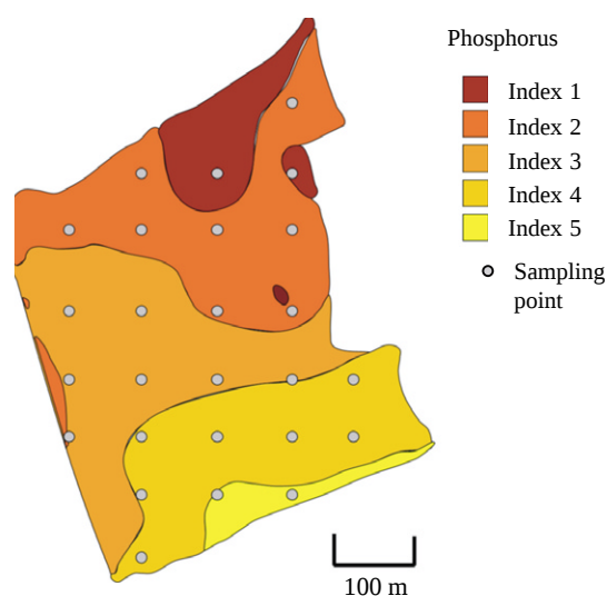
Fig. 14. Map of soil P (index values) derived from 100 m grid sampling (after Thomas et al. , 1999)
