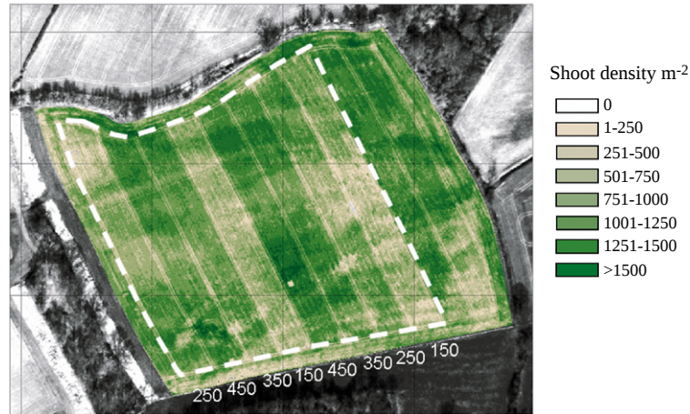
Fig. 16. Shoot density map derived from normalised difference vegetation index (NDVI), seed rated in seeds/m 2 are shown for the main strips (100 m grid) (after Taylor et al. , 2000)
