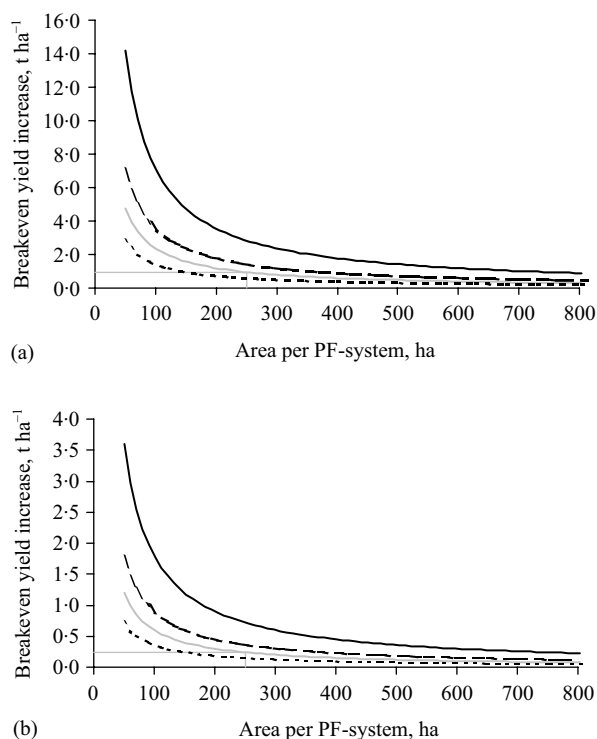
Fig. 7. Field variability sensitivity analysis for (a) class 3, and (b) class 4 systems, indicating the yield increase required on variable parts of the field to achieve breakeven at £65 t -1 for various areas of the field likely to produce positive response to variable inputs: —, 10%; ---, 20%; — · —, 30%; ·····, 50%.
