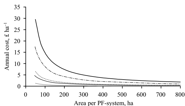
Fig. 1. Depreciation of the initial capital cost of precision farming (PF) equipment hardware for a class 1 system for a range of areas per PF-system: —, total hardware cost; ---, combine harvester; ·····, seed drill; — · —, fertiliser distributor; — — —, tractor
