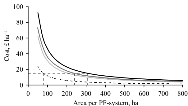
Fig. 6. Breakeven area for each of the 4 classes of precision farming (PF)-systems for a return of £15 \text{ha}^{-1} : ---, class 3; —, class 2; —, class 1; ·····, class 4; ·····, £15 \text{ha}^{-1}
