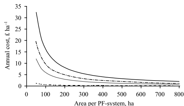
Fig. 2. Other associated costs of precision farming (PF) equipment for a class 1 system for a range of areas per PF-system: —, total associated cost; ---, cost of capital; ·····, maintenance; — · —, training
